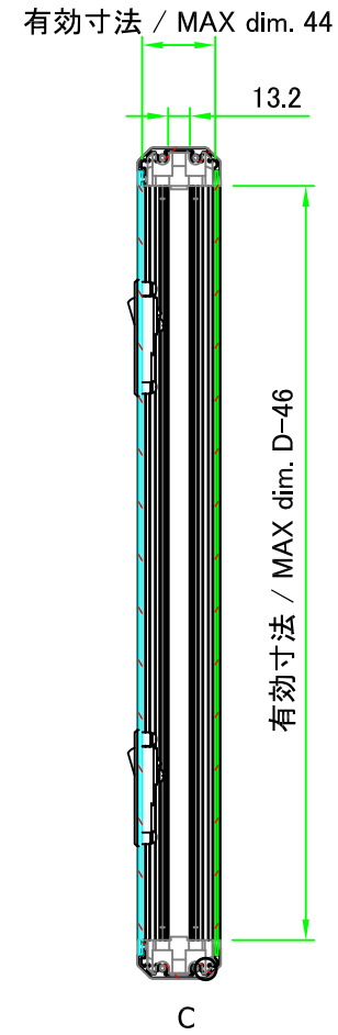
B-B (1:5)
